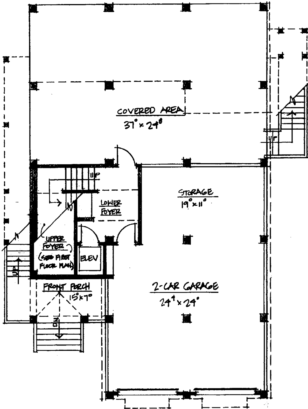
B503 - GROUND FLOOR
