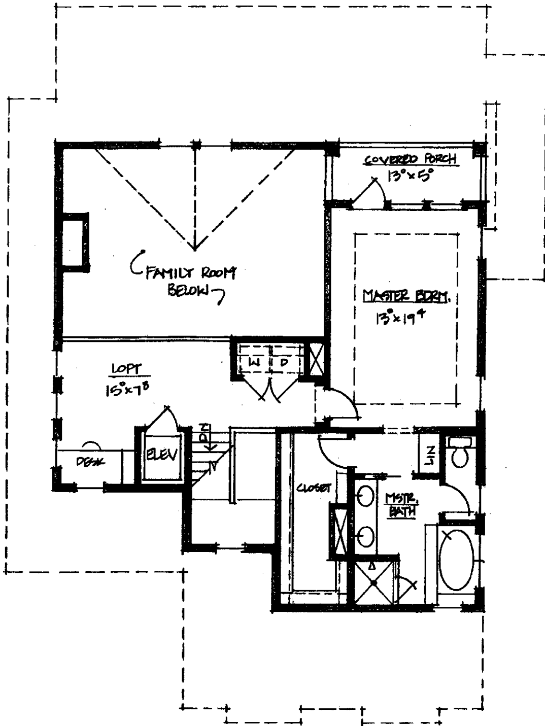
B503 - 2 ND FLOOR
