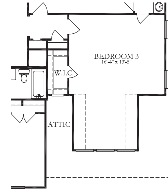
Option #0563 ENLARGED BEDROOM 3 From Attic + 106 sq.ft.
