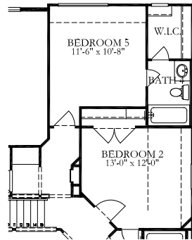
Option #0338 BEDROOM 5/ BATH 4 From Attic Space +218 sq.ft.
