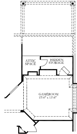
Option #0176 HIDDEN STORAGE/COVERED PORCH From Attic Space +50 sq.ft.
