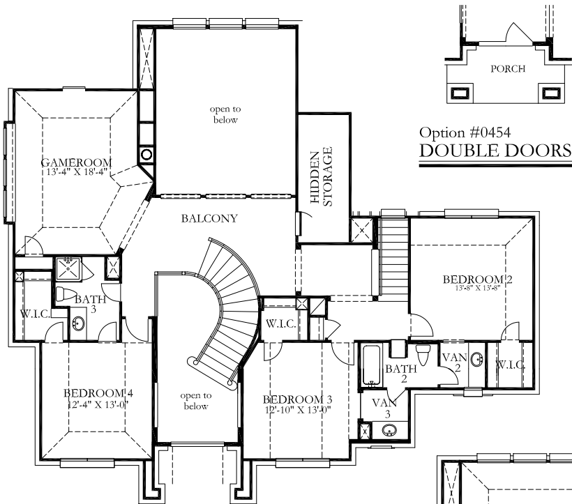
SECOND FLOOR
